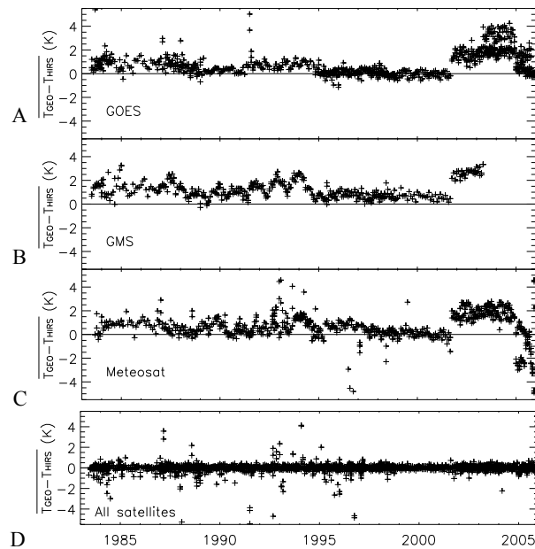
Fig. 2 - Initial monthly average difference between HIRS ( T_{\text{HIRS}} ) and geostationary ( T_{\text{GEO}} ) infrared window ( \sim 11\mu\text{m} ) brightness temperatures for A) GOES, B) GMS and C) Meteosat satellites. D) Monthly average difference after calibration correction for all satellite series.
