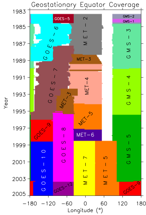
Figure 1 - Temporal and spatial Equatorial coverage from the geostationary satellites which make up ISCCP B1 data (shading is limited to a view zenith angle less than 60^\circ for illustrative purposes).
