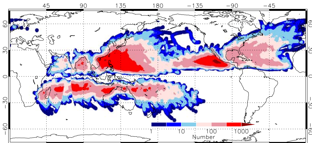
Fig. 3 - Spatial distribution of the number of observations within 250 km of a tropical cyclone for 1983-2005. The relatively data-void region in the S. Indian Ocean was not well-sampled until the Meteosat 5 coverage data began there in 1998.
